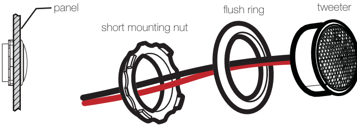
Fig. 5 Flush Mounting
