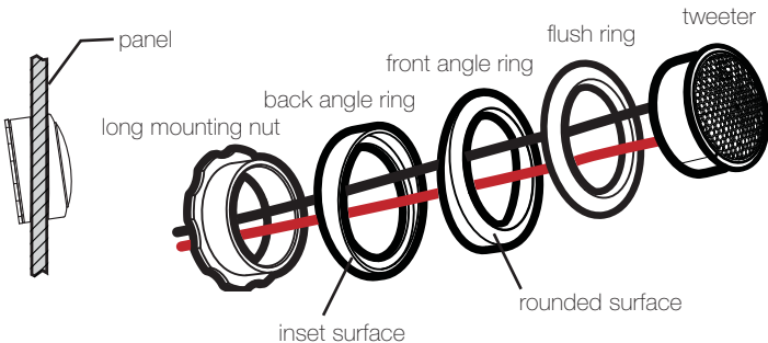
Fig. 6 Angle Mounting
