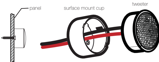
Fig. 7 Surface Mounting
